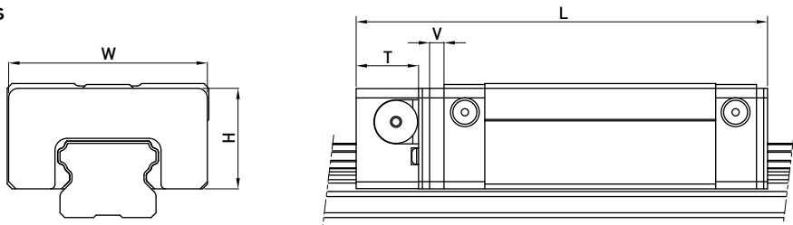
(6) QE Series
