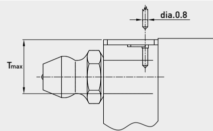
Size O-Ring Lube hole at top: max. permissible depth for piercing do (mm) W (mm) T max (mm) AG 20 4.5±0.15 1.5±0.15 5.7 AG 25 4.5±0.15 1.5±0.15 5.8 AG 30 4.5±0.15 1.5±0.15 6.3
