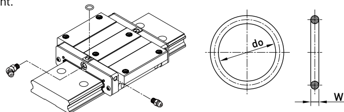
O Ring
