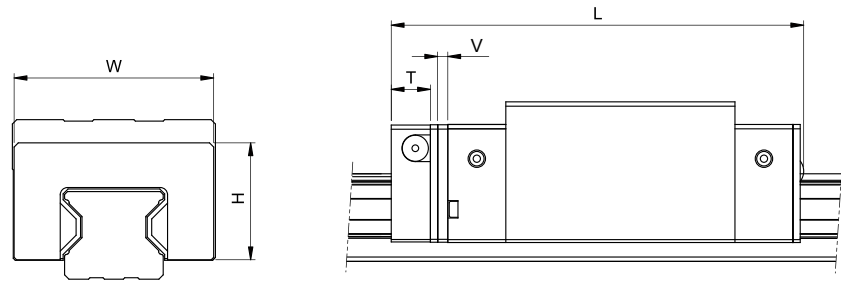
(5) QR Series
